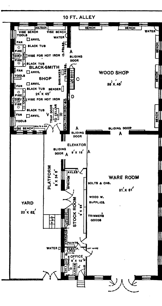
FIG. 27.—PLAN OF THE FIRST FLOOR.
