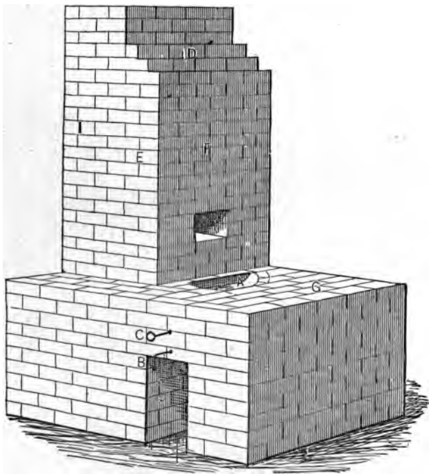
FIG. 14--AN IMPROVED FORGE.
