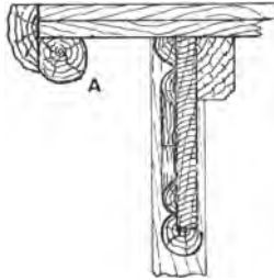
Fig. 100.—Section of Gable for Cottage Porch.
