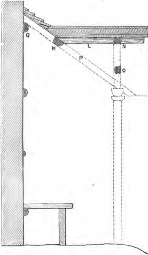
Fig. 161.—Section through Centre of Lean-to Summer-house.
