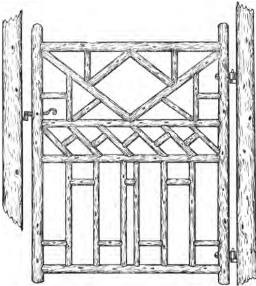
Fig. 86 —Alternative Design for Gate.
