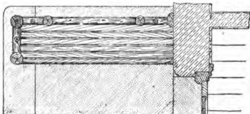
Fig. 96.—Part Plan of Seat and Floor of Cottage Porch.
