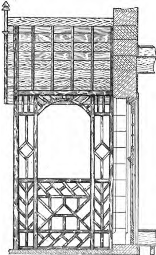
Fig. 95.—Vertical Section of Cottage Porch.
