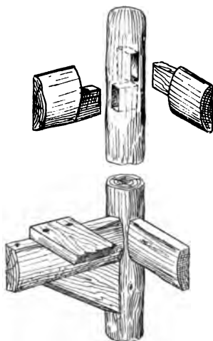
Fig. 19.—Fixing Rails, etc., to Posts.
