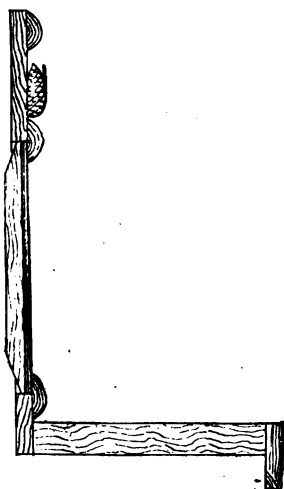
Fig. 2.—Section of Bracket, showing Fixing of Glass.
