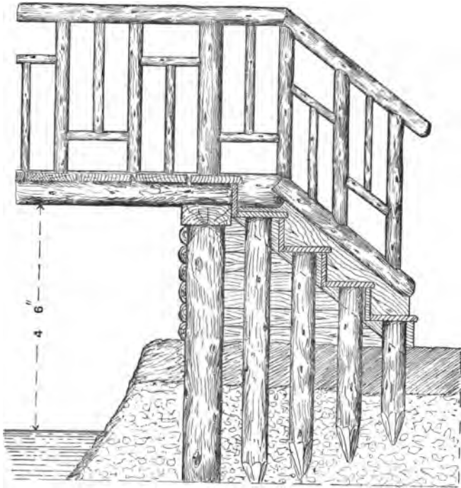
Fig. 130.—Elevated Foot-bridge.
