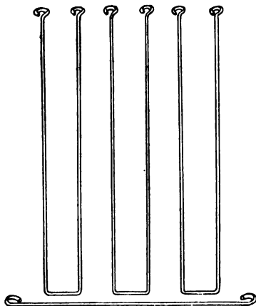
Fig. 118.—Construction of Door Wires for Aviary.
