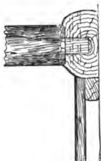
Fig. 103.—Fixing Middle Post of Canopy to Sill.
