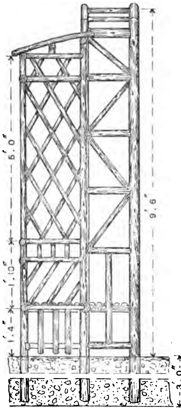
Fig. 83.—Vertical Section of Trellis
