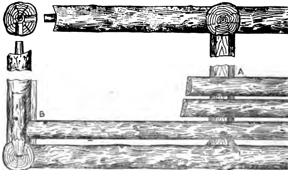
Fig. 152.—Detail of Seat of Garden Retreat.
