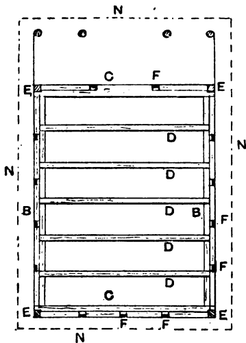
Fig. 143.—Plan of Ground Framework of Garden Snuggery.
