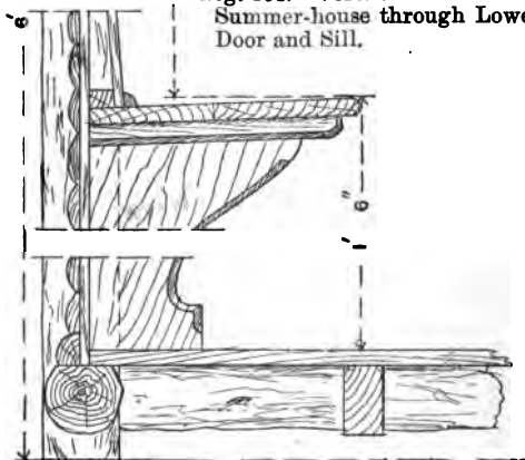
Fig. 183.—Vertical Section of Octagonal Summer-house through Side Casement.
