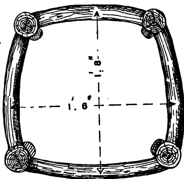
Fig. 48.—Plan of Armchair Seat Frame
