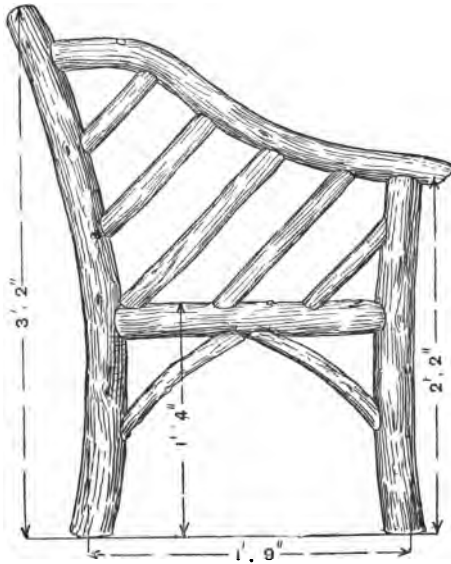
Fig. 50.—End Elevation of Garden Seat.
