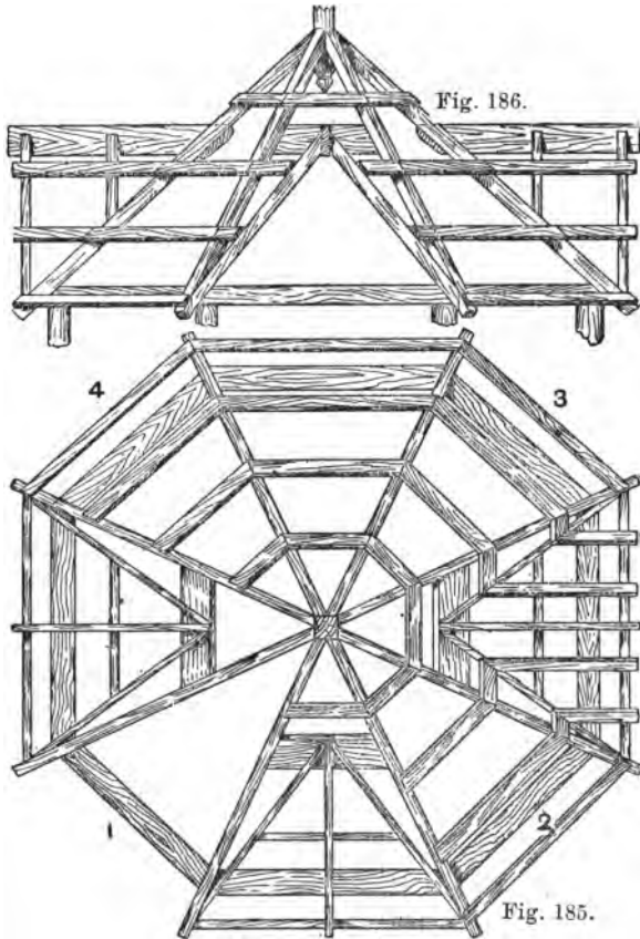
Figs. 185 and 186.—Elevation and Plan of Roof for Octagonal Summer-house.
