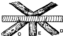
Fig. 28.—Fixing Centre Shelves of Flower-pot Stand.
