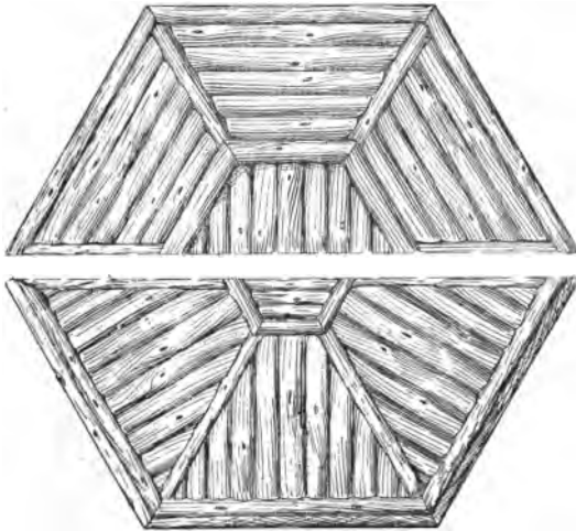
Fig. 45.—Half Plans of Top of Hexagonal Table.
