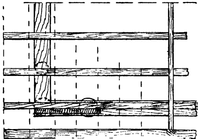
Fig. 99.—Part Plan of Roof for Cottage Porch.
