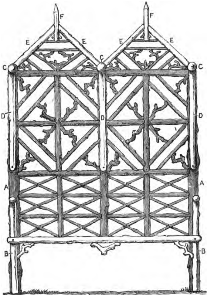
Fig. 59.—Front Elevation of Garden Seat.
