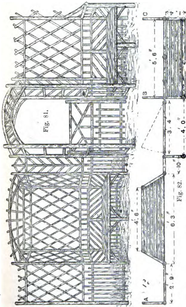
Figs. 81 and 82 —General View and Ground Plan of Rustic Trellis with Seats and Gate.
