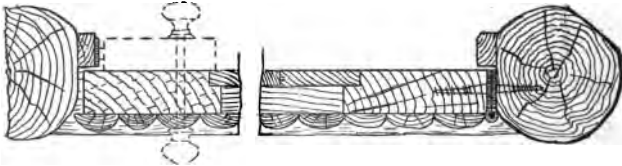
Fig. 191.—Horizontal Section through Door Posts,
