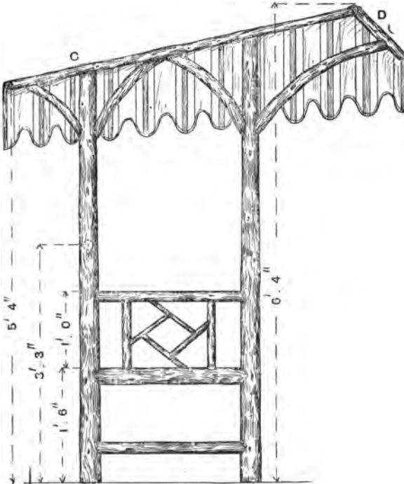
Fig. 151.—Side Elevation of Garden Retreat.
