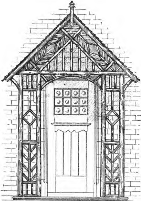
Fig. 94.—Front Elevation of Cottage Porch.
