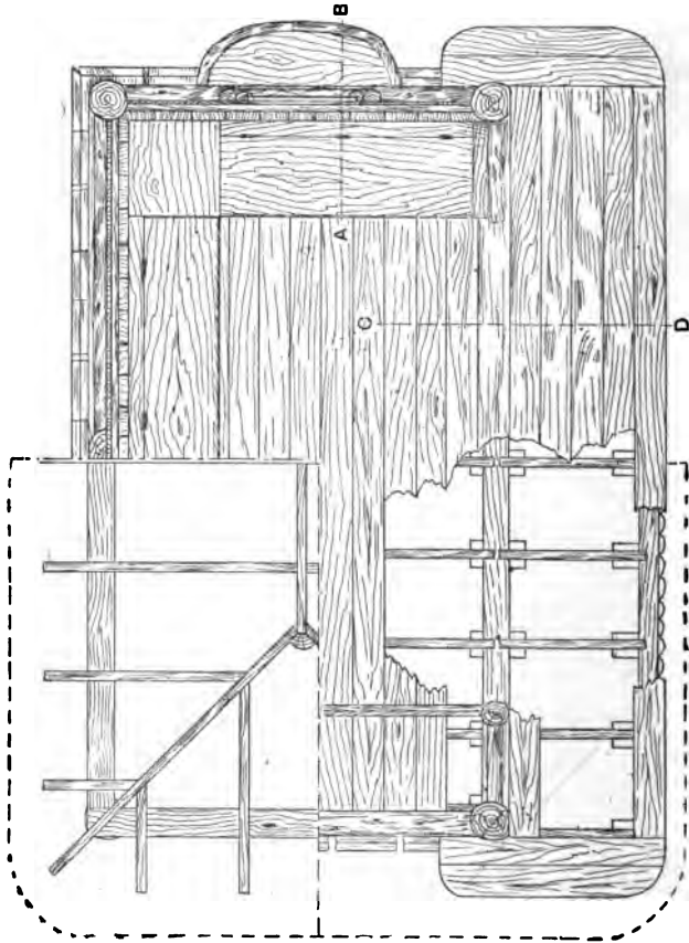
Fig. 164.—Part Roof, Seat, and Floor Plans for Tennis Lawn Shelter.
