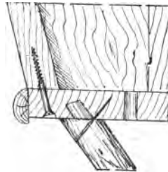
Fig. 22.—Securing Sides and Legs of Vase to Base.
