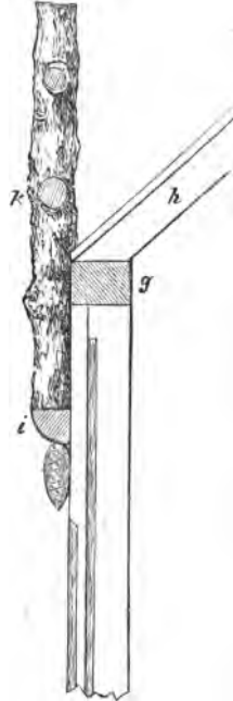
Fig. 136.—Side View of Top of Post for Glazed Verandah.
