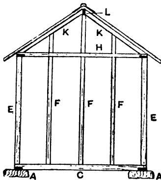
Fig 144.—Back Framework for Garden Snuggery. H
