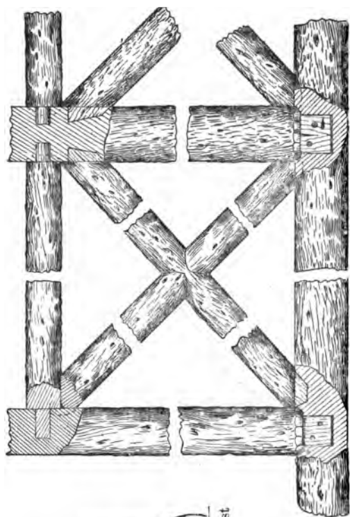
Fig. 103.—Fixing Middle Post of Canopy to Sill.
