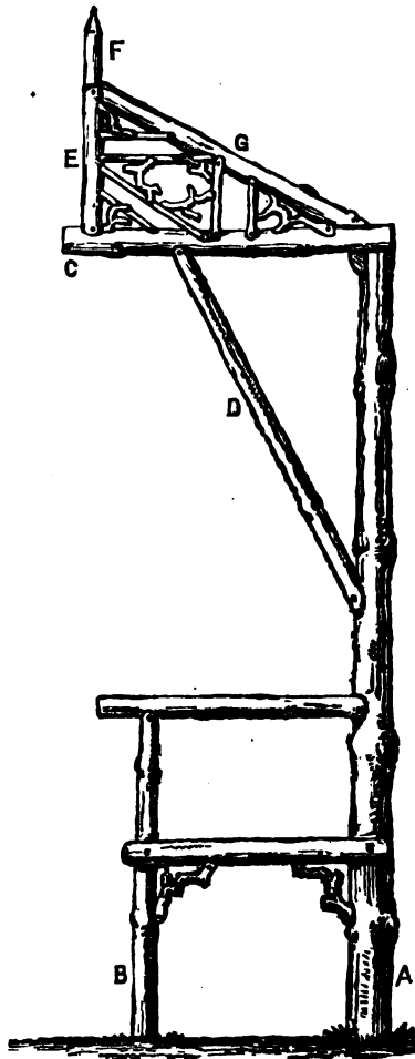
Fig. 60.—End Elevation of Garden Seat.
