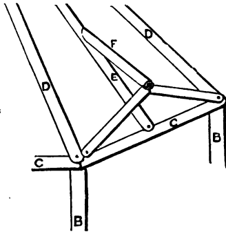
Fig. 176.—Timbers over Entrance of Octagonal Summer-house.
