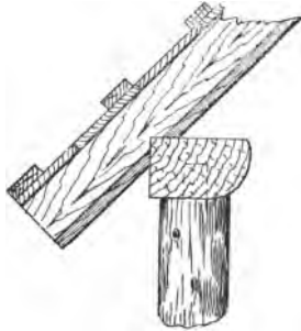
Fig. 98.—Enlarged Detail of Cottage Porch at Eaves.
