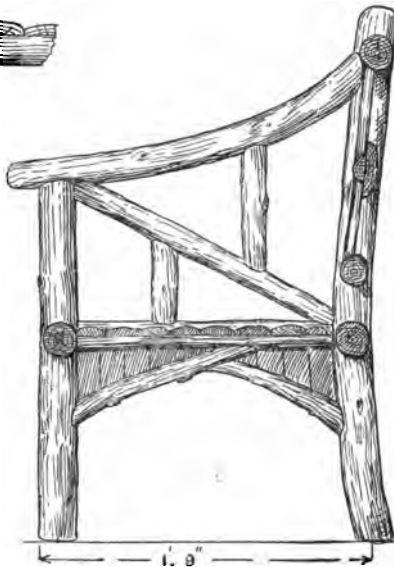
Fig. 55.—Cross Section of Garden Seat.
