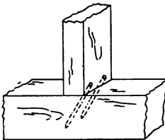
9 Toe-nailed
