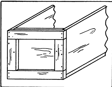
Fig. 283. Reinforced Butt Joint in Box.
