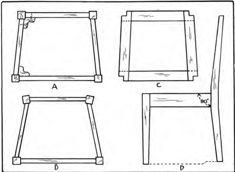
Fig. 298. Chair Construction.
