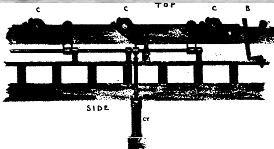
Fig. 44. Automatic Steam Transfer for Timber, Lumber and Slabs. The boards are carried along by the cylinders, C C C, until they hit the bumper, B. This movement admits steam to the cylinder, CY, which raises the revolving chains or skids, which transfers the stock sidewise to other live rollers as required.
