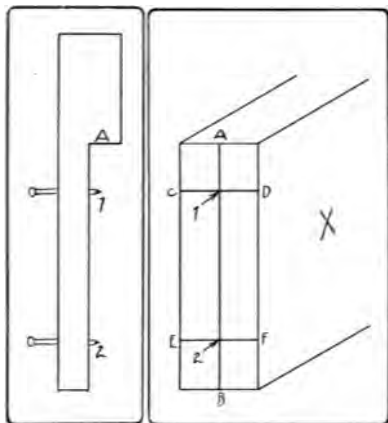
Fig. 249. Laying out a Dowel Joint.
