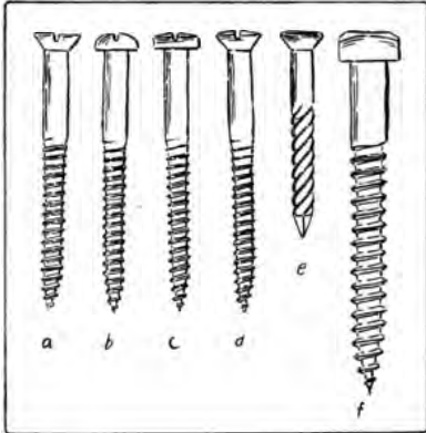
Fig. 229. a. Flat-head Wood-screw. b. Round-head Wood-screw. c. Fillister-head Wood-screw. d. Oval-countersunk-head Wood-screw. e. Drive-screw. f. Square-head (lag-or-coach-) Screw.
