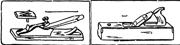
Fig. 99. Adjustable Chisel-Gage. Fig. 100. Wooden Bench-Plane.
