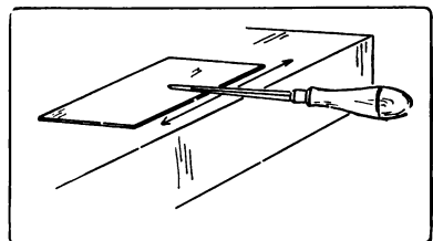
Fig. 157. Resharpening a Cabinet-Scraper: Flattening the Edge.
