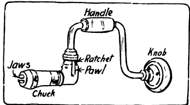
Fig. 185. Ratchet-Brace.
