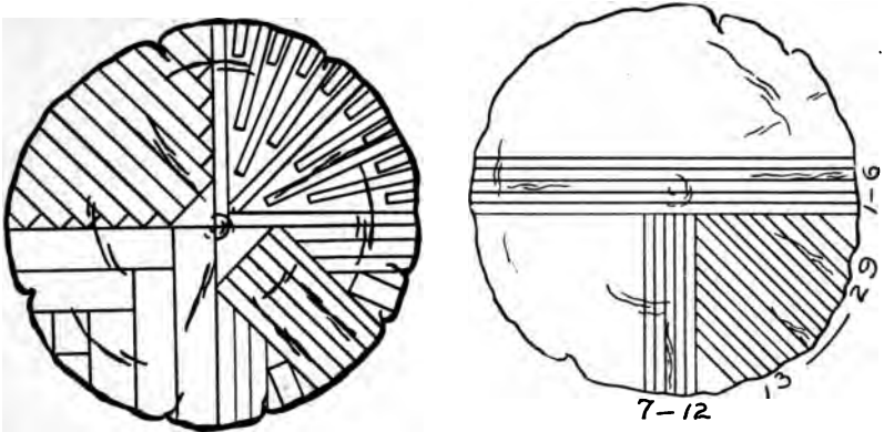
Fig. 56. Methods of Sawing Quartered Logs.
