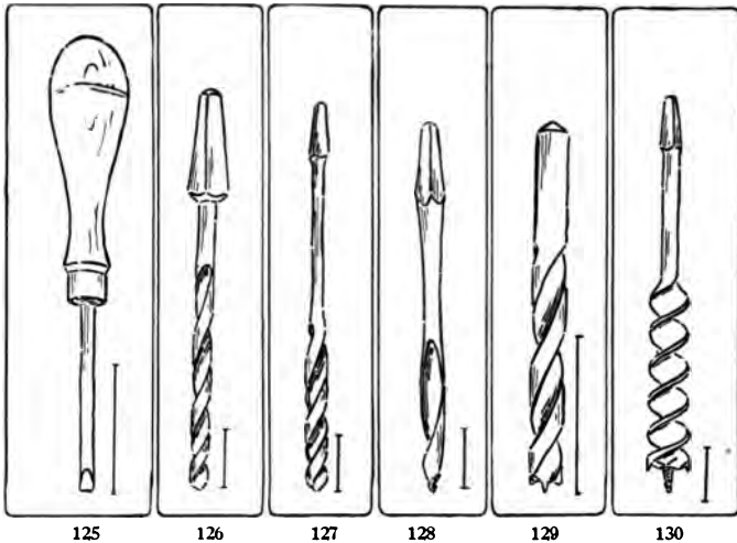
Fig. 125. Brad-Awl. Fig. 126. Twist-Drill. Fig. 127. Twist-Bit. Fig. 128. German Gimlet-Bit. Fig. 129. Bit-Point Drill. Fig. 130. Auger-Bit.
