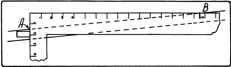
Fig. 300 A. Method of Laying Out Better of Side Rail of Chair.
