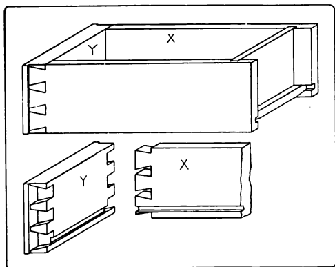
Fig. 287. Dovetailed Drawer Construction.
