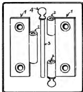
Fig. 234. Parts of a butt-hinge. 1.1. Leaves. 2.2.2. Knuckle. 3. Pintle. 4. Acorn.
