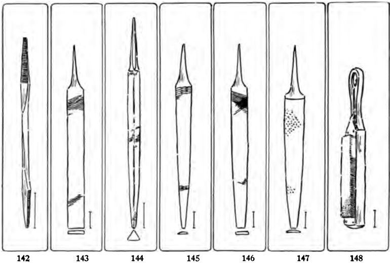
Fig. 142. Auger-Bit-File.
