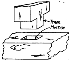
30 Stub mortise-and-tenon
