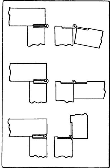
Fig. 235. Three Positions of Hinges.
