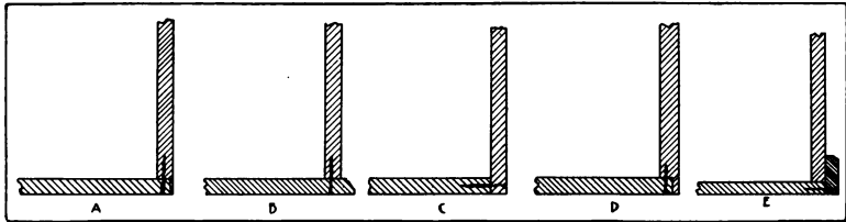
Fig. 284. Methods of Attaching Box Bottoms.
