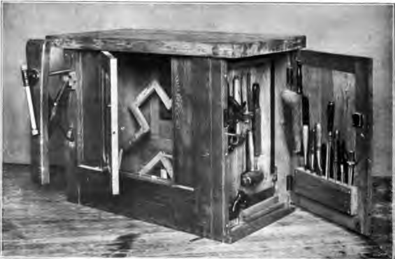
Fig. 167. Woodworking Bench Used at Pratt Institute, Showing Self-Adjusting Upright Vise.
