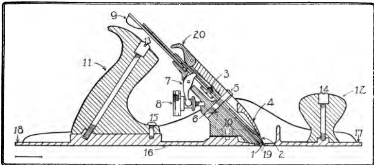
Fig. 101. Section of Jack-Plane.
