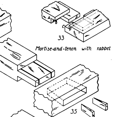
35 Wedged mortise-and-tenon
