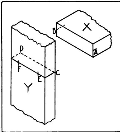
Fig. 246. Lay-out for Thru Doweling.
