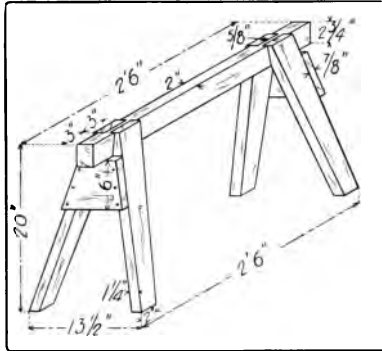
Fig. 170. Saw-Horse.
