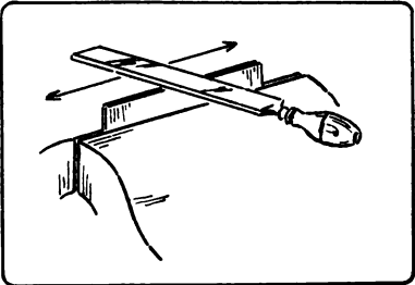
Fig. 153. Sharpening a Cabinet-Scraper: 1st Step, Drawfiling.
