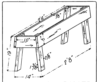
Fig. 171. Saw-Horse.
