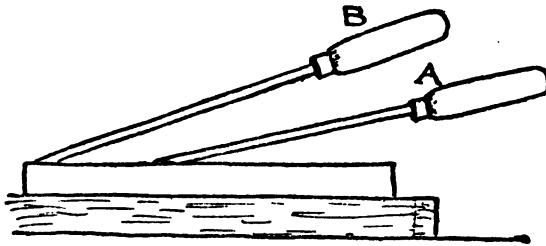
A. ANGLE FOR SOFTWOOD B. ANGLE FOR HARDWOOD
